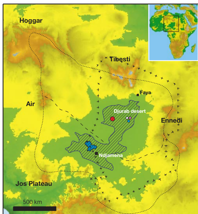
Figure 1 Map of the Chad basin showing the location of the Toros-Menalla area. The crossed line represents the Chad border. The boundaries of the ancient Lake Chad basin are shown as a dotted line (with northern and southern sub-basins divided by a dashed line). The inferred maximum extension of the Holocene 'Lake Mega Chad' is hatched in black; the small blue area within it corresponds to present-day Lake Chad. Red circle, the Toros-Menalla hominid site (TM 266); white circle, the Kossom-Bougoudi area; pink circle, Kollé area; blue circle, Koro-Toro area. Colours represent altitude: green, 280–430 m; yellow to grey, 430–850 m; brown, 850–2,000 m; grey-blue patches in Tibesti area, about 2,000–3,400 m.
